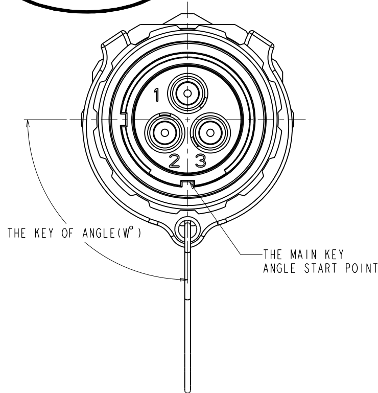
1,2,3 HOLES FOR POWER PIN
