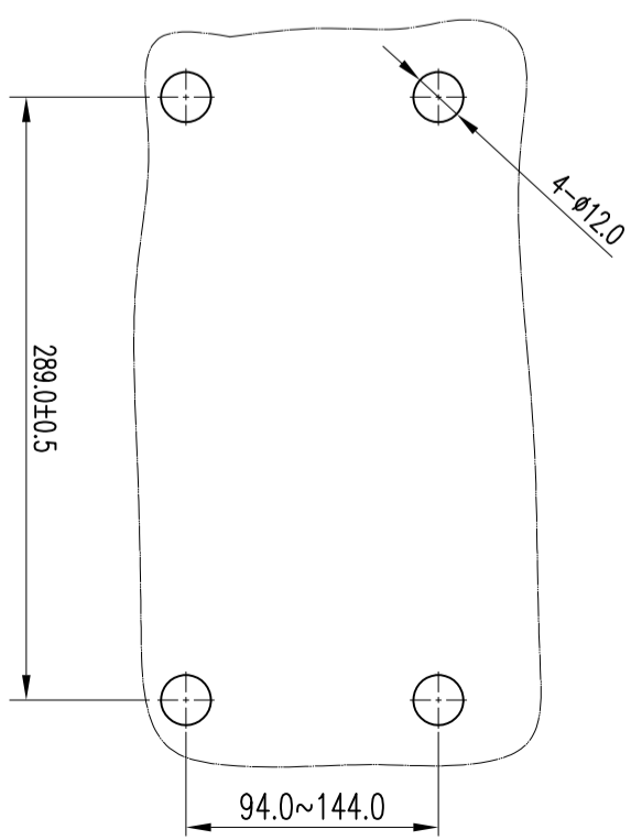
RECOMMEND PANE DIMENSION SCALE: 1:4
